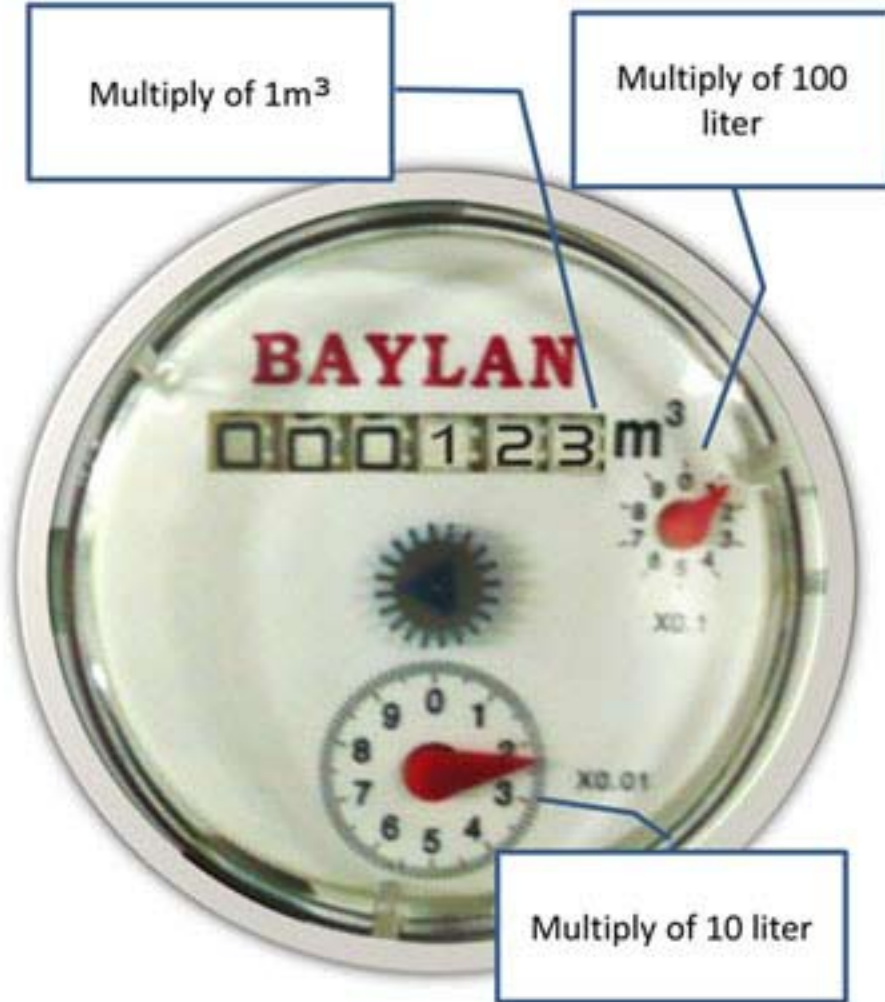
DN-65, DN-80, DN-100, DN-125 (W0, W1, W2, W3) Type Water Meters
