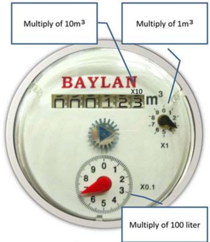
DN-150, DN-200 (W4, W5) Type Water Meters
