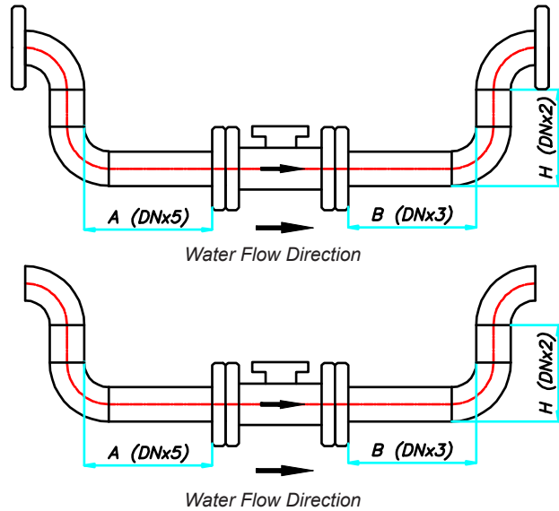
DN50-DN200 Ultrasonic Meters Installation
