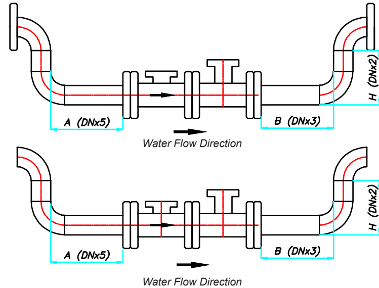
DN50-DN200 Ultrasonic Valve Meters Installation
